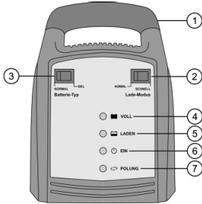
Figure 1: View of front
